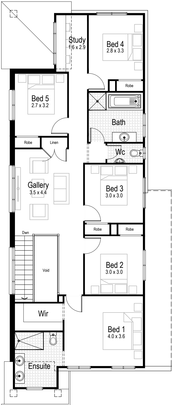
First Floor
