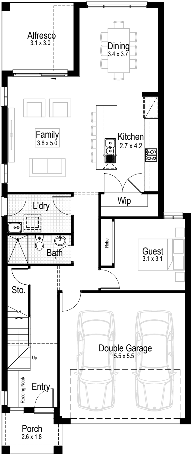
Ground Floor
